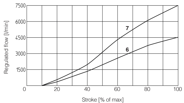
6 = LIQZA-LES-80* 7 = LIQZA-LES-100*
