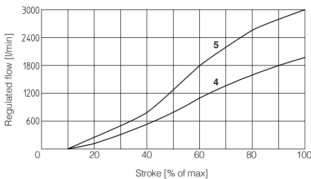
4 = LIQZA-LES-50* 5 = LIQZA-LES-63*
